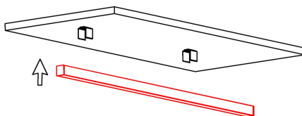
5. Mounting the profile with clip .
