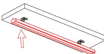
A5. Mounting the profile with clips
