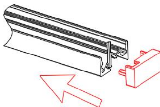
A5. Mounting the profile with clips
