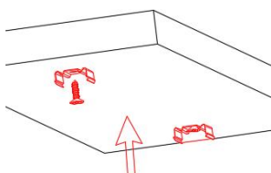
A4. Mounting the clips with screws
