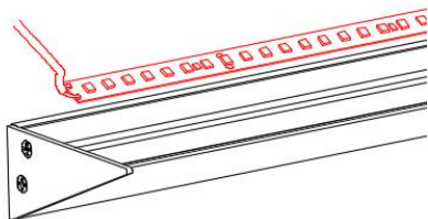
4. Stick the LED strip
